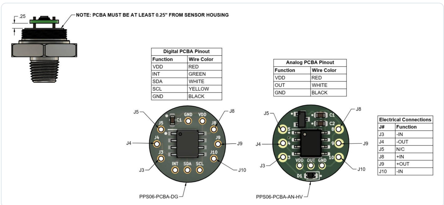
Fig. 1 – PCBA mounting (at least 0.25" from housing) and pinouts: PPS06-PCBA-DG (digital) and PPS06-PCBA-AN-HV (analog).
