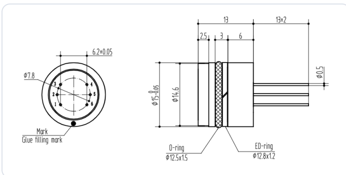
Fig. 2 – Uncompensated element, pin side view and profile (mm). 5-wire open bridge.
