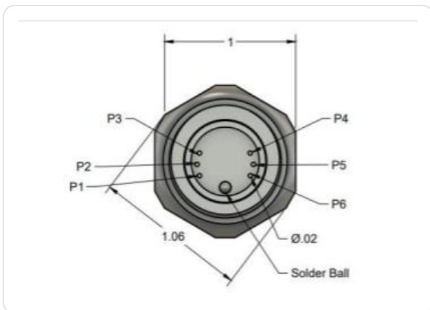
Fig. 3 – Pin positions P1-P6, viewed from pin side. The glue-fill mark (solder ball) sits below pins 1 and 6.
