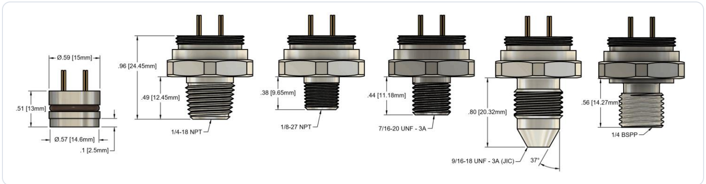
Fig. 4 — Sensor-only element (left) and threaded port housings: 1/4-18 NPT, 1/8-27 NPT, 7/16-20 UNF-3A, 9/16-18 UNF-3A (JIC), 1/4 BSPP.
