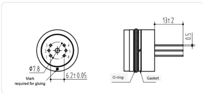
Fig. 1 – Compensated element, pin side view and profile (mm). 4-wire bridge.
