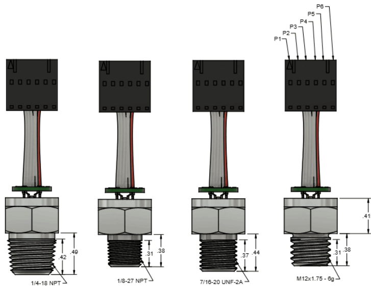
Fig. 5 – Left to right: 1/4"-18 NPT, 1/8"-27 NPT, 7/16"-20 UNF-2A, M12x1.75-6g, shown with ribbon cable and connector. 9/16"-18 UNF drawing available on request.
