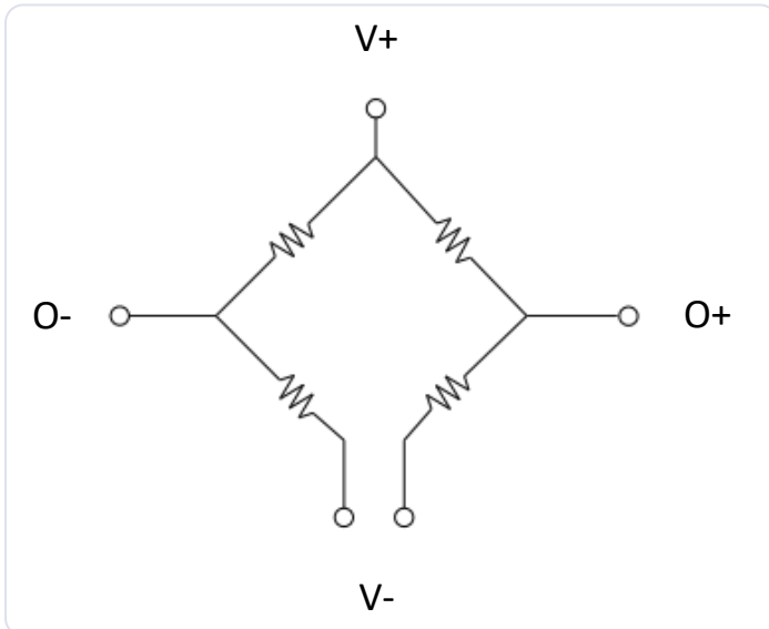
Fig. 2 – Bridge schematic with element pin assignments.
