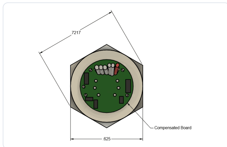
Fig. 3 – Compensation board inside the 0.625" port hex.
