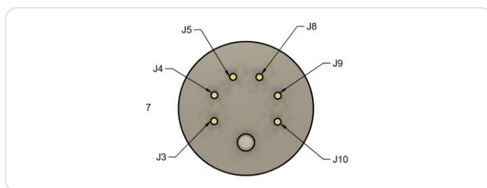
Fig. 1 – Element rear view showing pin positions J3–J10.
