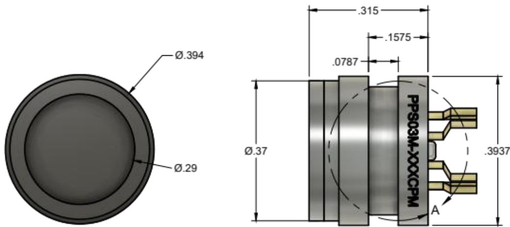
Fig. 4 – Diaphragm face (left) and side view (right). Height without pins: 0.315" (0.310–0.320).
