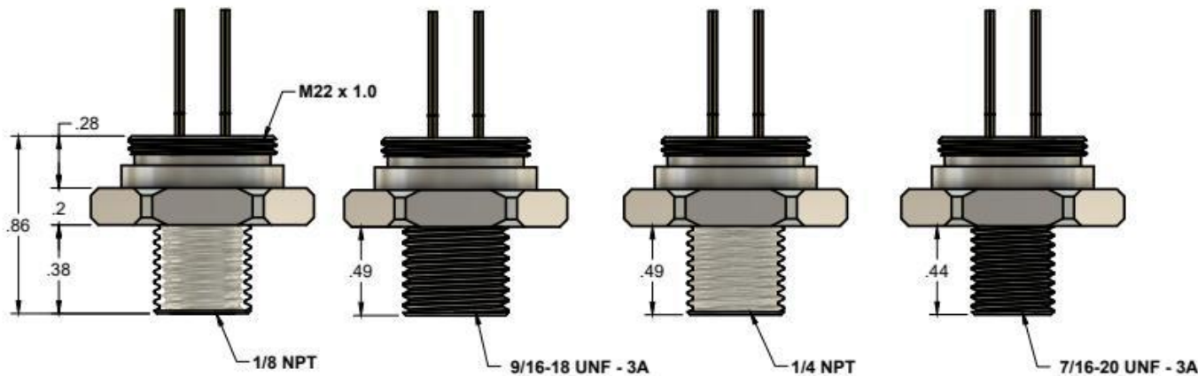
Fig. 2 — Sensor only (top); 1/8"-27 NPT, 9/16"-18 UNF, 1/4"-18 NPT and 7/16"-20 UNF ported versions with M22 × 1.0 mounting thread (bottom).
