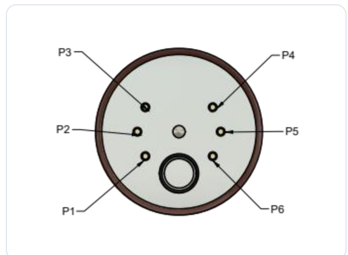
Fig. 1 – Pin layout viewed from the pin side. Gold-plated pins.
